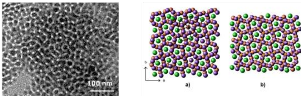
Figure 1. Cryo-TEM image of an ordered cluster of coated \text{CeO}_2 -NPs and its schematic representation.
