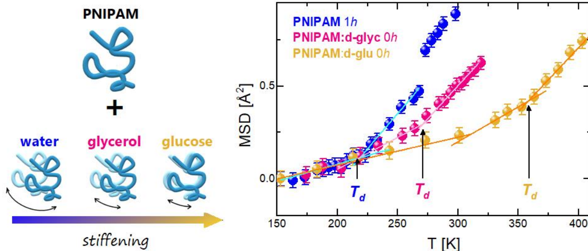
Figure 1. Mean square displacements (MSD) of PNIPAM in pure water (PNIPAM 1h), pure glycerol (PNIPAM:d-glyc 0h) and pure glucose (PNIPAM:d-glu 0h). According to the characteristics of the employed spectrometer (IN13), the reported MSD are associated with motions faster than \tau_R=150 ps. For each sample, the activation of the DT at the corresponding value of T_d is indicated with an arrow.
