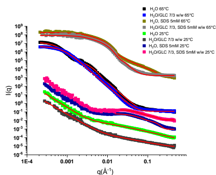
Figure 1. SANS scattering profiles at 25 and 65°C.
