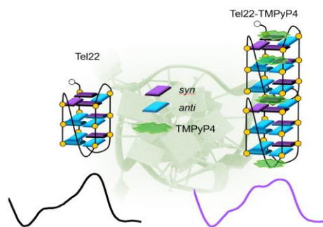
Figure 1. Schematic view of Tel22 before and after binding with TMPyP4.
