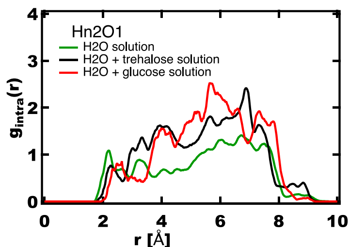
Figure 2. Comparison of the intra-molecular g_{\text{Hn2O1}} , sites involved in the β-turn formation, in the three GPG-NH 2 solutions, namely in pure water (green line) 5 , in a water-trehalose solution (black line) 5 and in the water-glucose solution investigated here (red line) 6 .
